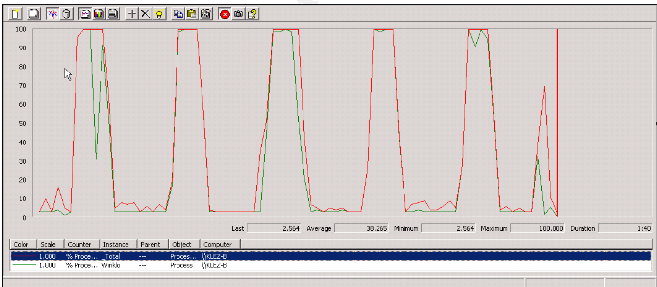
Figure 2. Total CPU Utilization (red) versus Winklo process CPU utilization (green)
