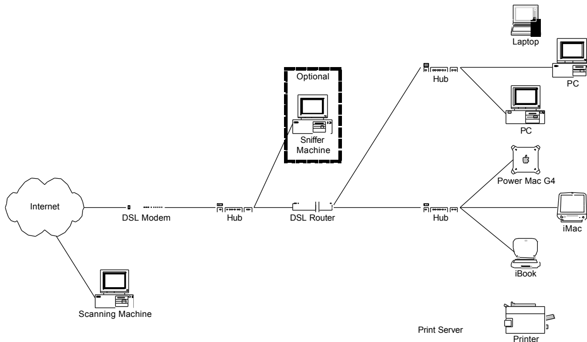
Figure 3 Example Network Diagram for Testing the DSL Router Configuration via the Internet
